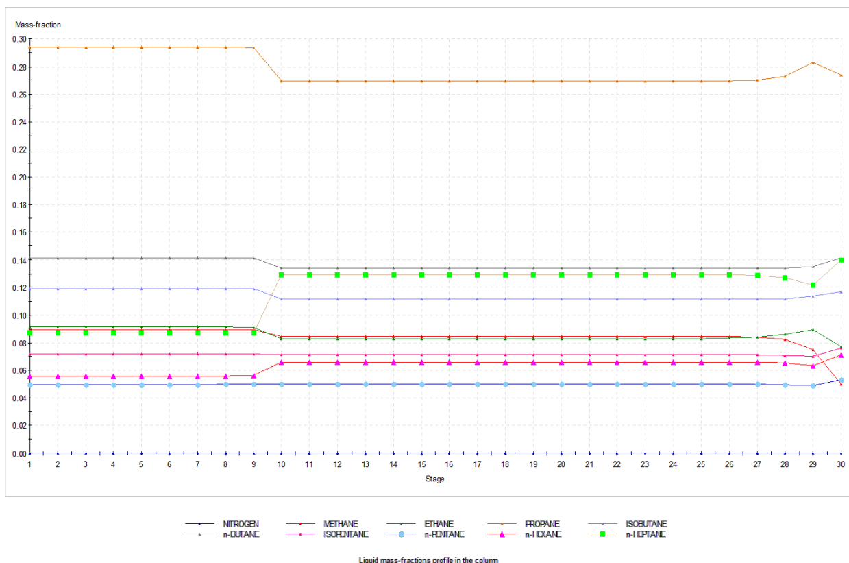
Liquid mass-fractions profile in the column
