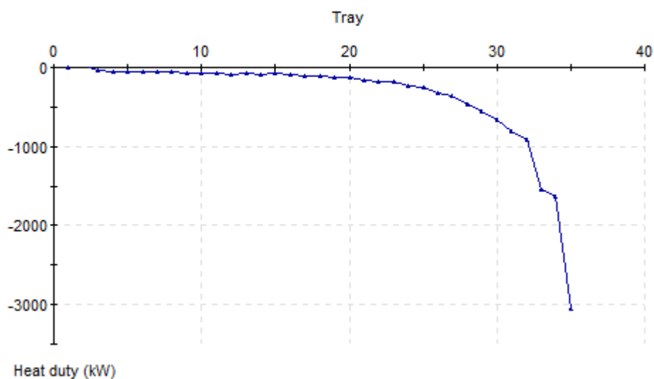
C101 - Heat duty
